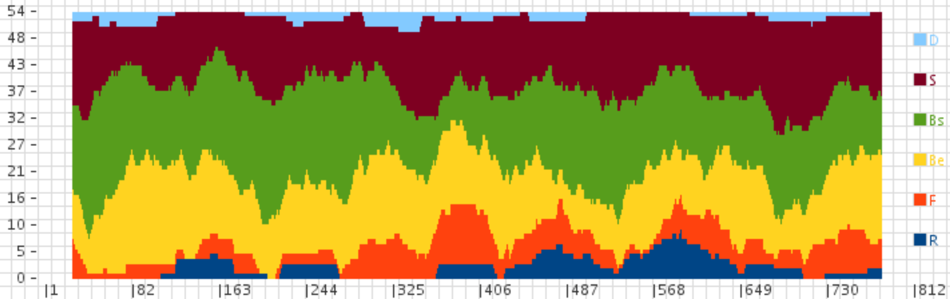
Dynamic issues from segment 1 to 811 and a window of 54 segments.
